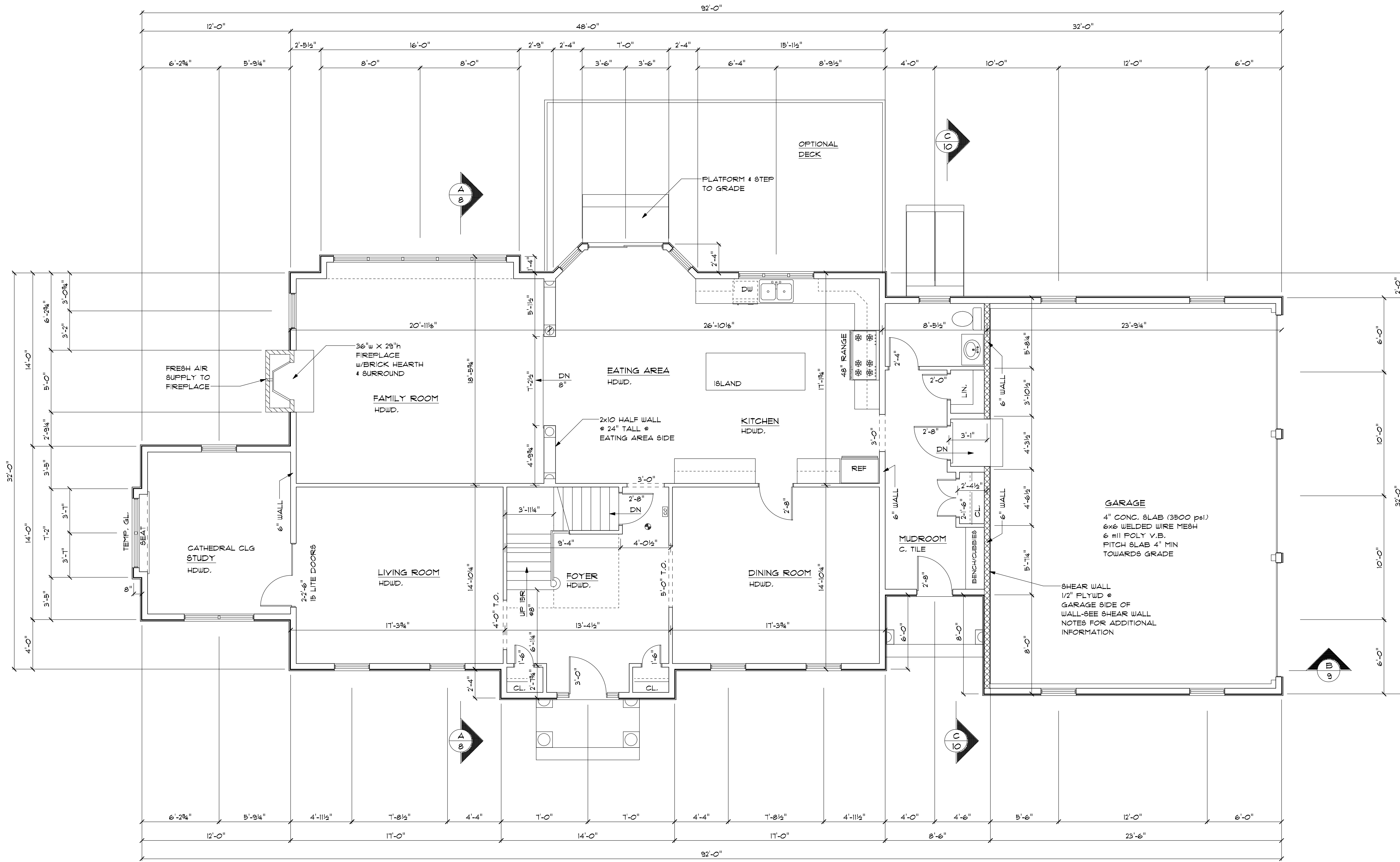
FIRST FLOOR PLAN +/-1979 sq.ft.
